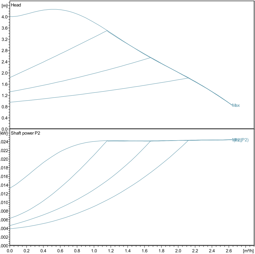
Performance according to ISO 9906:2012 – Grade 3B Liquid temperature: Power data referred to: Water, pure [100%]; 4°C; 1000kg/m³; 1.57mm²/s
